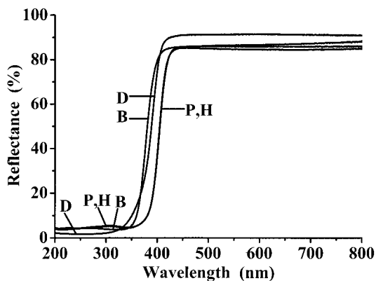
Figure 6 Reflectance spectra of four TiO 2 powders.
